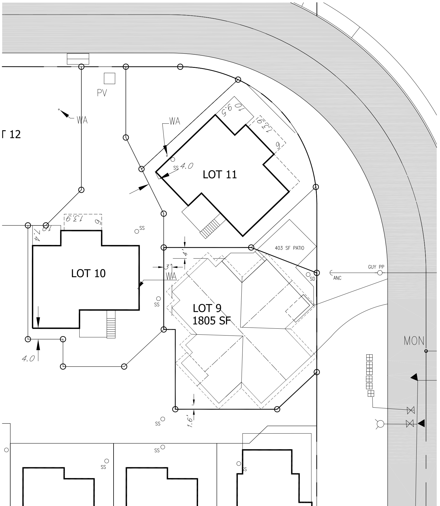
PROPOSED OUTLINE - 1805 SF RAMBLER LOT 9 - THE ISLES
